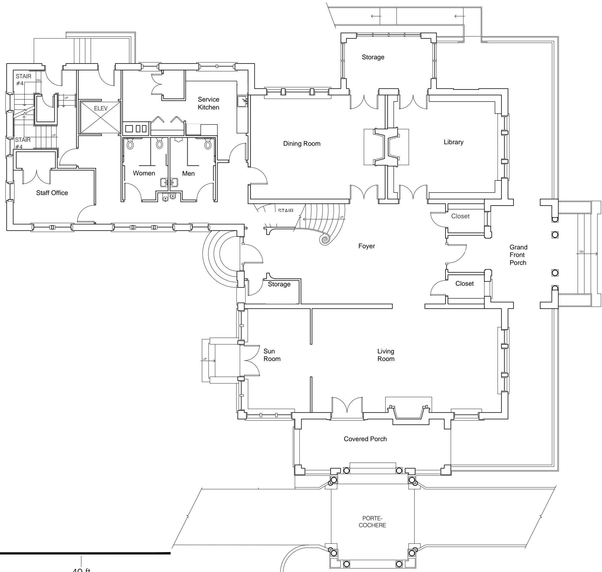
Lord Mansion First Floor Plan
